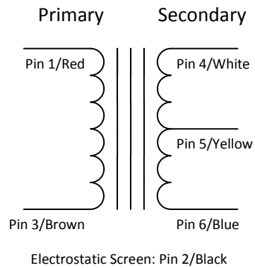
Pinout
