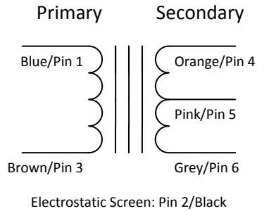
Pinout
