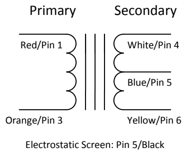
Pinout
