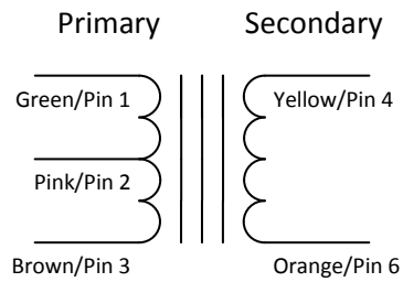
Pinout
