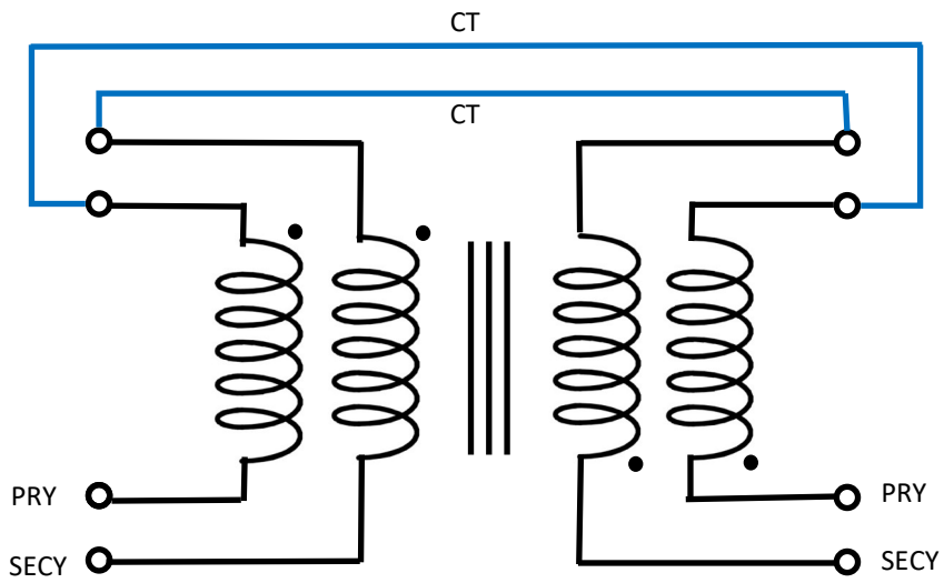
Wiring for Push-Pull operation
