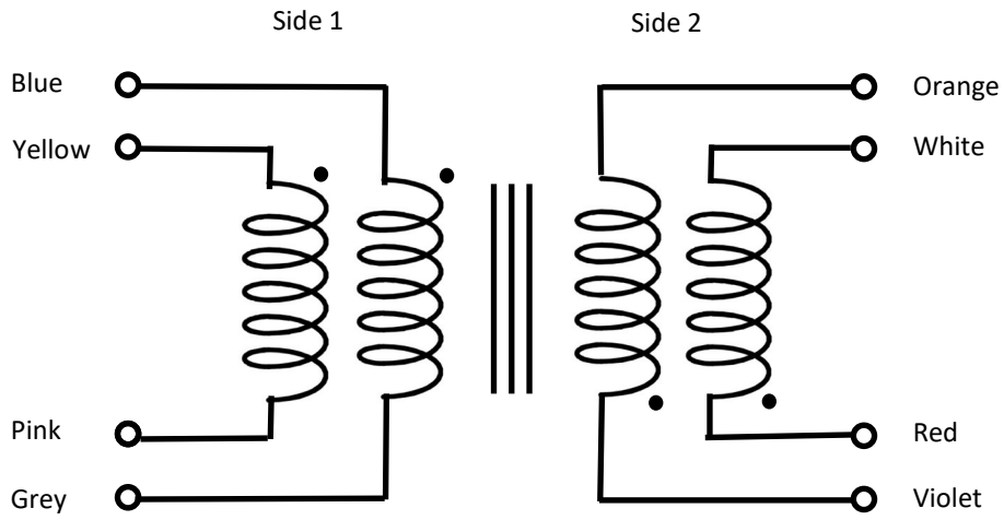
Bifilar wound double bobbin
